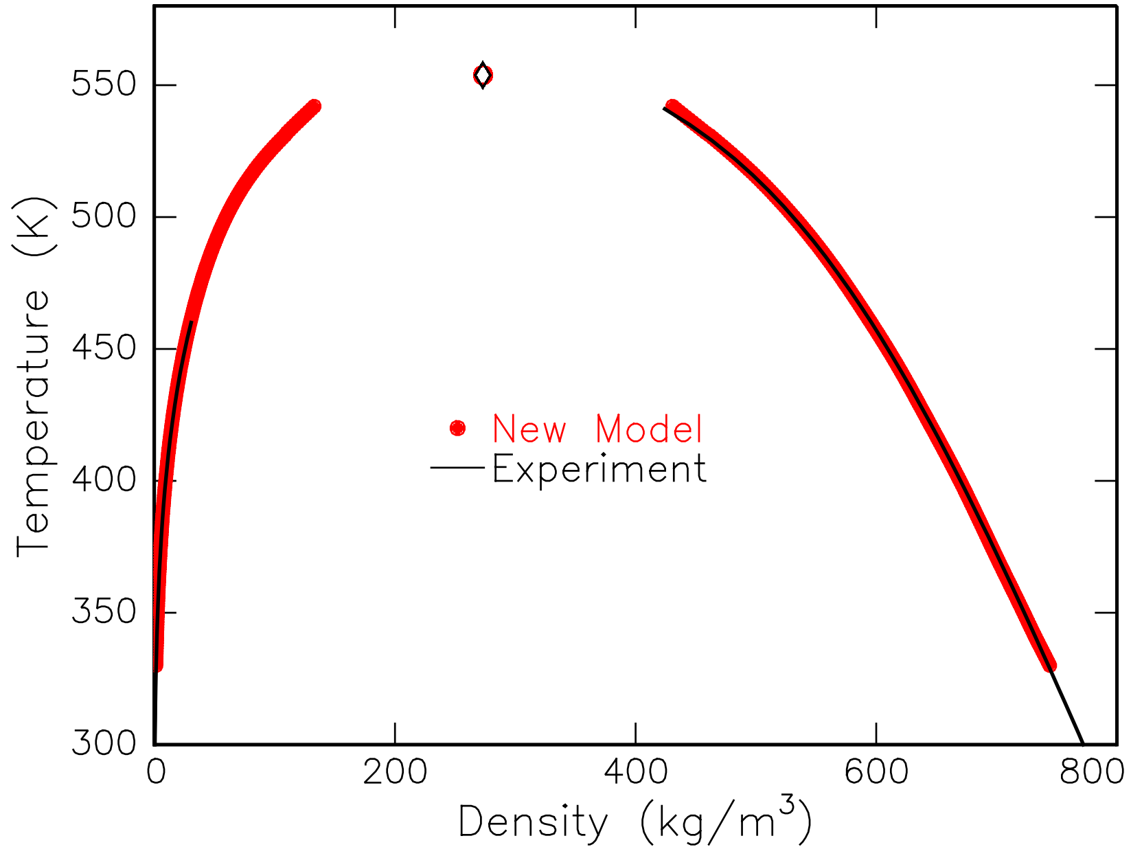
c-Hexane Coexistence Curve
