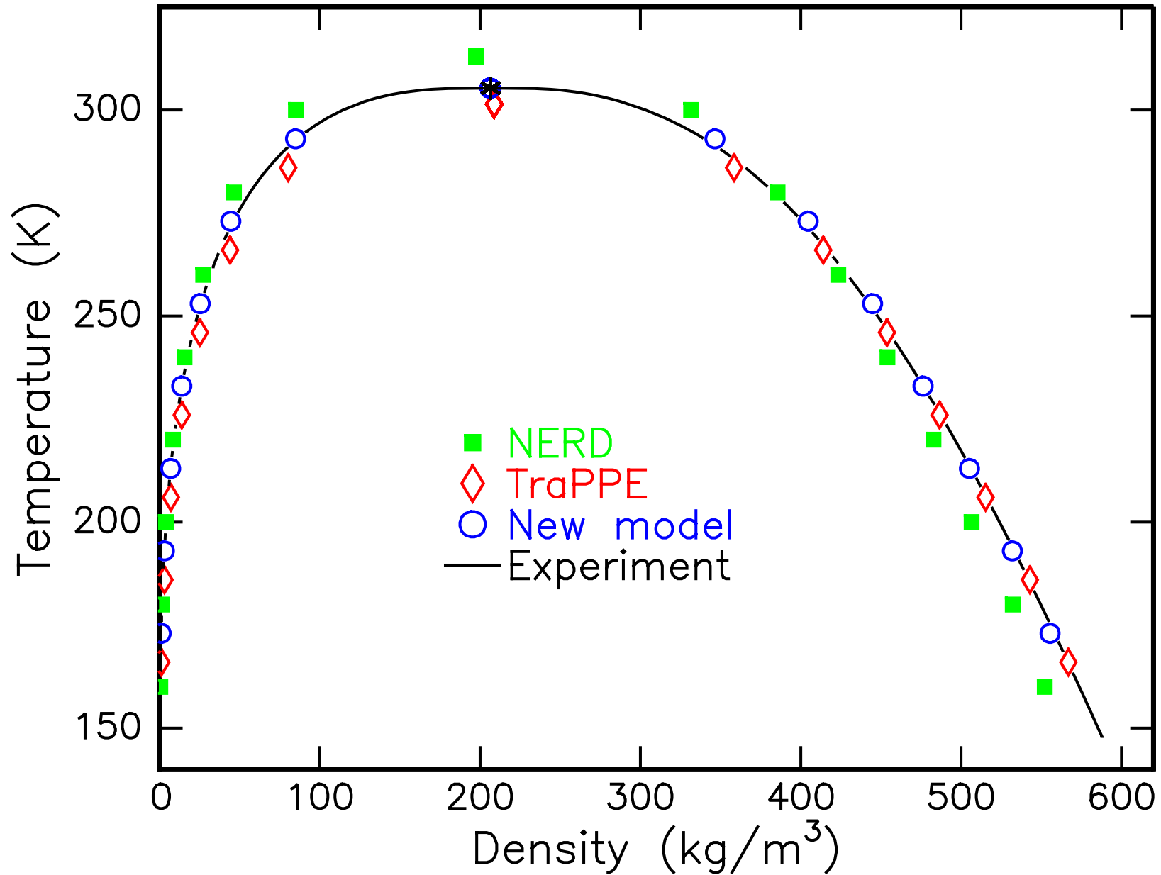
Ethane Coexistence Curve
